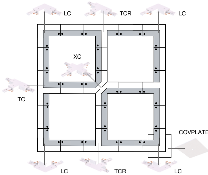
Loop type run with connection from L connector
