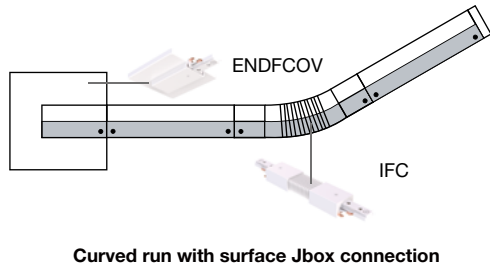
Curved run with surface Jbox connection
