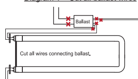
Diagram 1 – Cut all ballast wires
