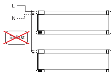
Diagram 4 – Multiple tube wiring
