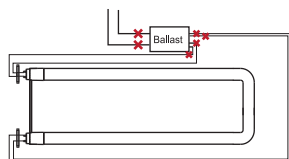
Diagram 5 – Cut all ballast wires
