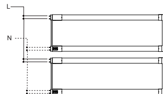
Diagram 8 – Multiple tube wiring
