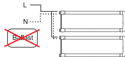
Diagram 4 – Multiple tube wiring
