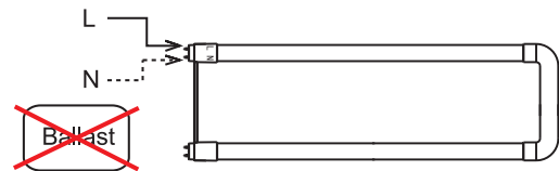
Diagram 3 – Single tube wiring
