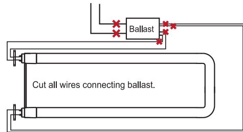
Diagram 1 – Cut all ballast wires
