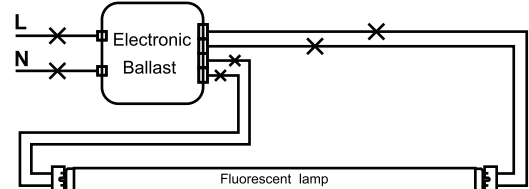
Programmed Start or Rapid Start (Non-shunted socket) Configuration
