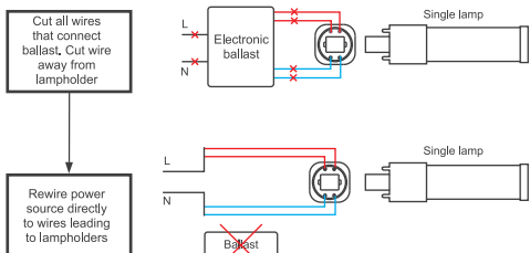
Diagram 2 – Electronic ballast fixture wiring modification
