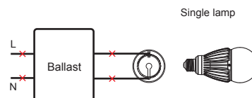
Diagram 2 – Fixture with ballast wiring modification
