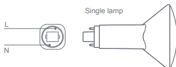
Diagram 1 – New fixture without ballast wiring
