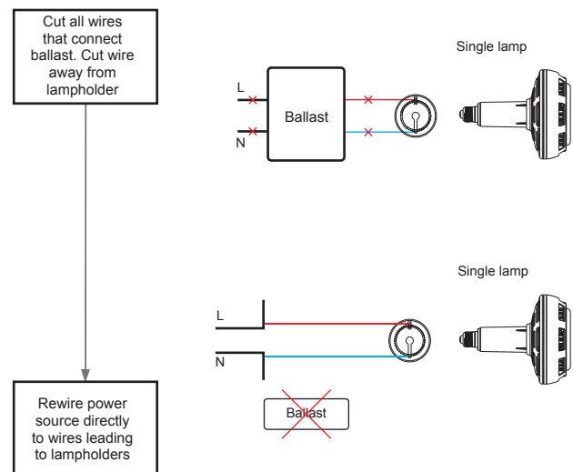
Diagram 2 – Fixture with ballast wiring modification
