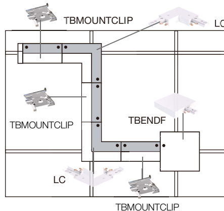
S type run with T-bar ceiling end feed
