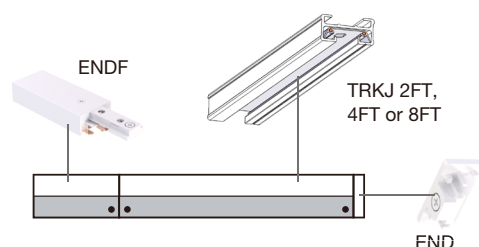
Linear run with end feed connection
