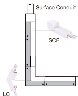
L type run with surface conduit connection
