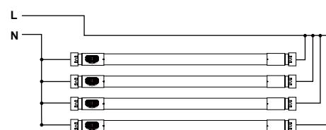
Multiple Lamps Maximum 4 tubes should be interconnected.
