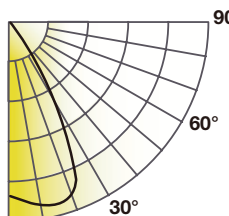
LES9035-DIM010-UNV-MD-ADR8CC
