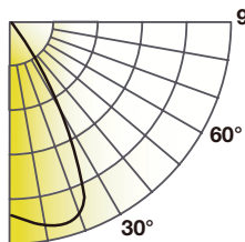
LEM9035-DIM010-UNV-MD-ADR8CC
