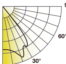
LES9035-DIM010-UNV-WD-ADR8CC
