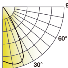
LEL9035-DIM010-UNV-MD-ADR8CC
