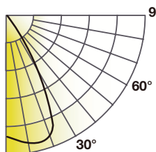
LES9035-DIM010-UNV-MD-ADR8CC
