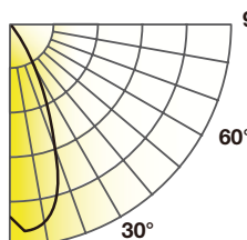
LES9035-DIM010-UNV-NR-ADS6CC
