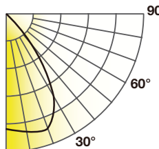
SPFST6-LEL9035-KDIM010-UNV-WD-ADS6CC
