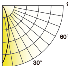
SPFST6-LES9035-KDIM010-UNV-VN-ADS6CC
