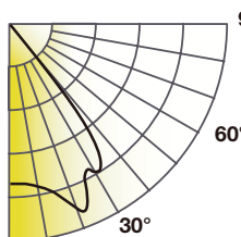
SPFTR6-LEM9035-KDIM010-UNV-WD-ADR6CC
