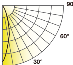
SPFTR6-LES9035-KDIM010-UNV-VN-ADR6CC
