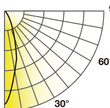
SPFTR6-LEM9035-KDIM010-UNV-VN-ADS6CC
