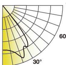
SPFTR6-LES9035-KDIM010-UNV-WD-ADR6CC
