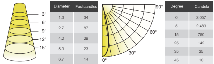
6.5GU10DIM/930NF25
