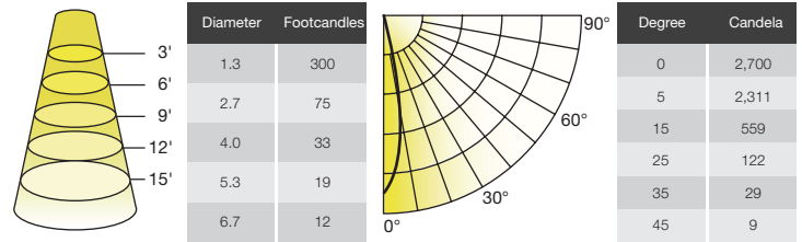
7.5MR16DIM/930NF25/R, 7.5MR16DIM/930NF25/RC
