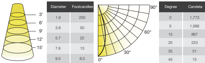
6.5GU10DIM/930FL35
