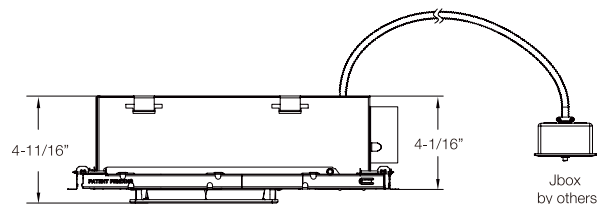
4" and 6" Square S Lumen Shallow IC Frame Cover with EM6 (shown with 6" Light Engine)
