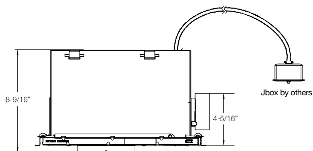
6" and 8" Round M Lumen Large IC Frame Cover with EM6 (shown with 6" Light Engine)
