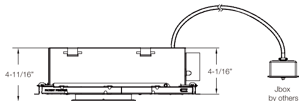
4" , 6" and 8" Round S Lumen Shallow IC Frame Cover with EM6 (shown with 6" Light Engine)
