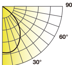
NYXNC8RD/S9CCT5S/DUALDIM/WD/CC (3500K Selected)
