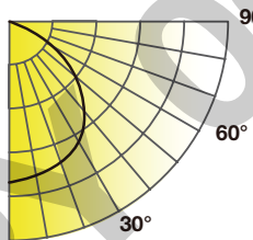
SLFTG3/8/9CCT5S/DUALDIM (at 3500K)
