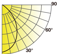
SLFTG3/6/9CCT5S/DUALDIM (at 3500K)
