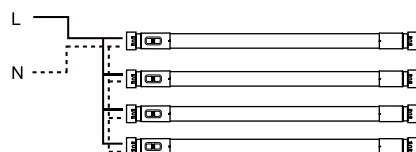
Programmed Start or Rapid Start (Non-Shunted Lamp Holders)
